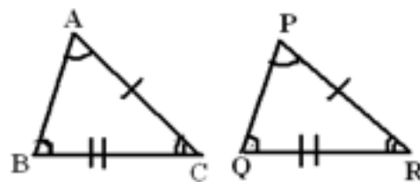
Congruence of triangles
